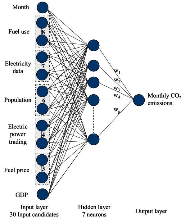
Fig. 2 Architecture of RBFN reference model.
