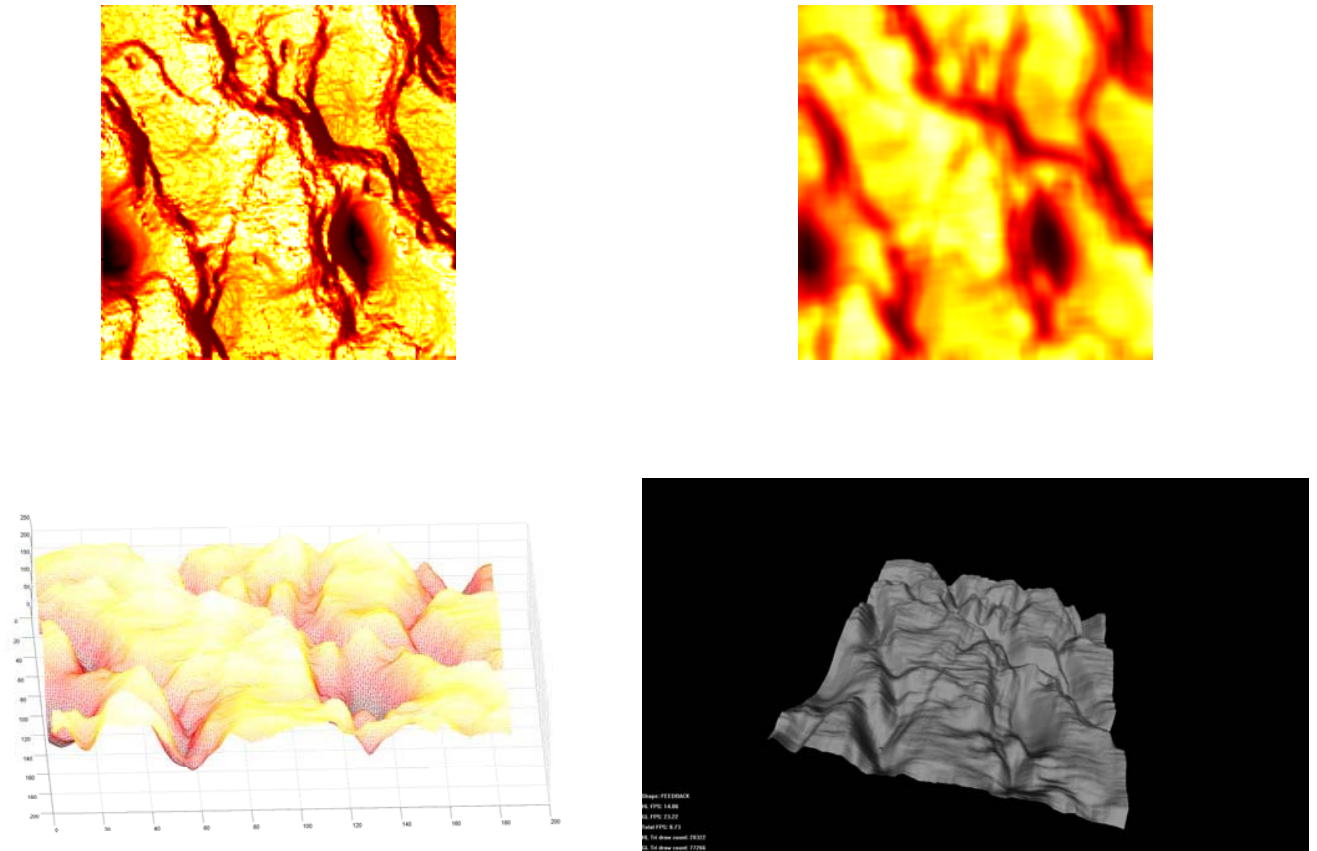
Fig. 7. top-left: Raw AFM image of the scanned sample, top-right: Filtered version of raw Image (left), Bottom-left: Rendered surface of the ltered image (top-right), Bottom-right: Generated virtual Haptics surface
