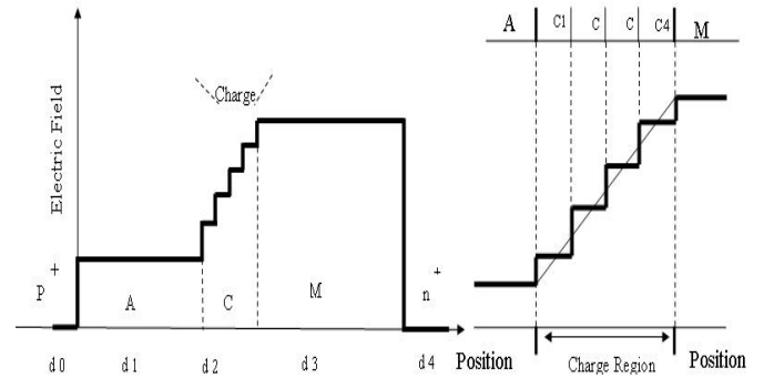
Fig.3. Implementation of split-step method in charge region
