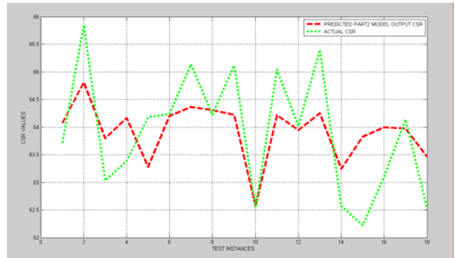
Fig. 7 NN Output For Coke Process Prediction Model
