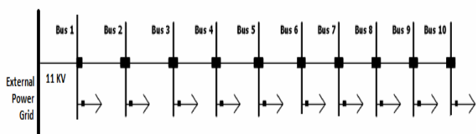
Fig. 2 11 KV Radial Feeder
