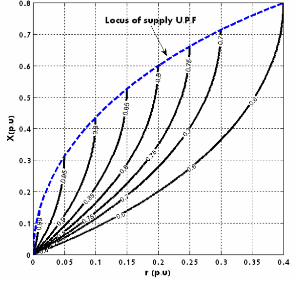
Fig. 6 Relation between \Delta P (or r_1 ) and x_2 for different values of load power factor
