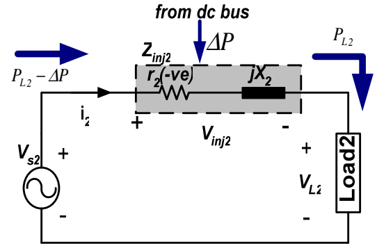
Fig. 7 Feeder 2 circuit with virtual impedance injection
