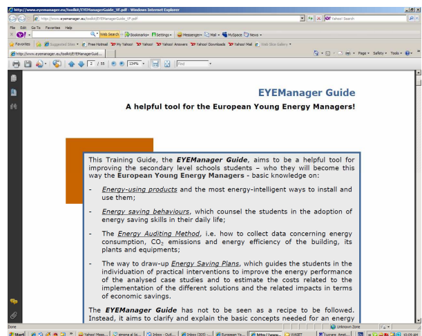
Fig. 3 EYEManager Guide
