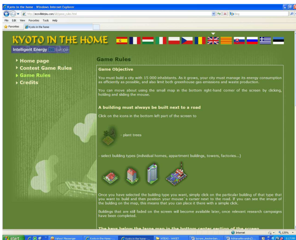
Fig. 4 Ecoville Game
