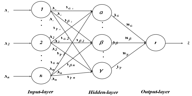
Fig. 4 Framework of a three-layer neural network
