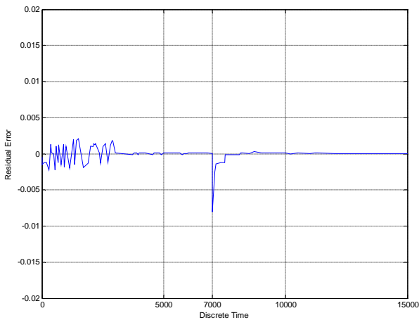
Fig. 11 Residual error generated from the linear observer after the motor driven gain fault.
