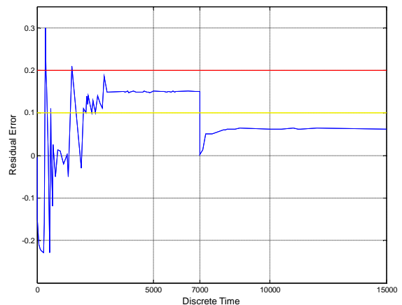
Fig. 10 Residual error generated from the dynamic neural network after the motor driven gain fault.
