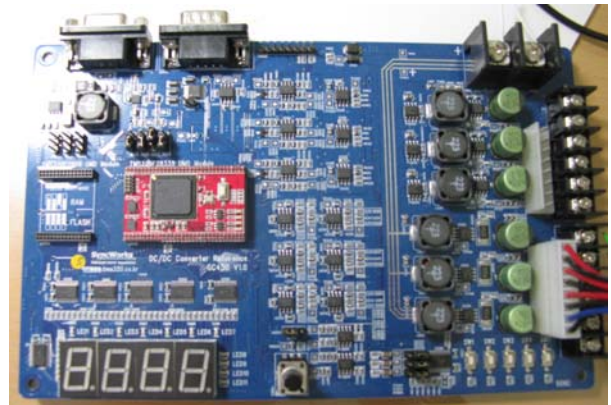
Fig. 9 Control Board
