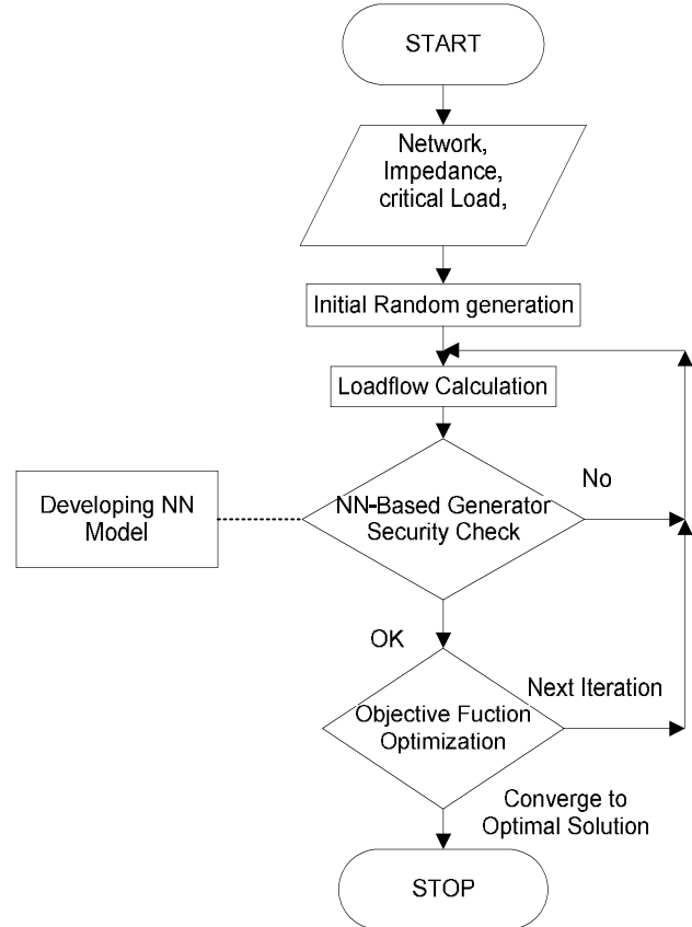
Fig. 2 IPSO based OPF Flowchart
