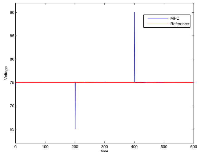
Fig. 5: Constant voltage control based on MPC
