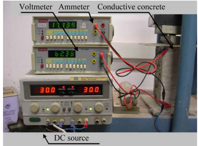
Fig. 2. Measured diagram of the press-electrode method.
