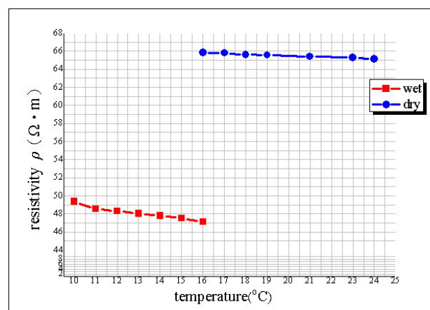
Fig. 4. Relation curve of resistivity and temperature in press-electrode method.
