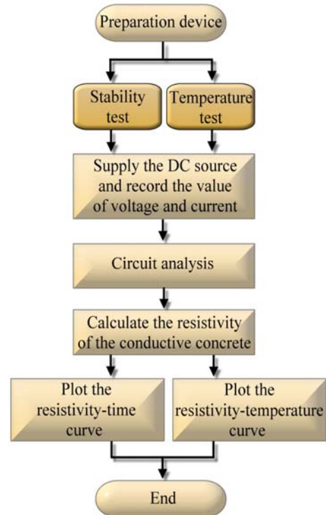
Fig. 3. Flowchart of the resistivity measurement.
