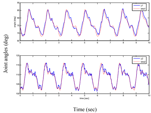
Fig. 6. Response of NN controller: actual and desired joint angles.
