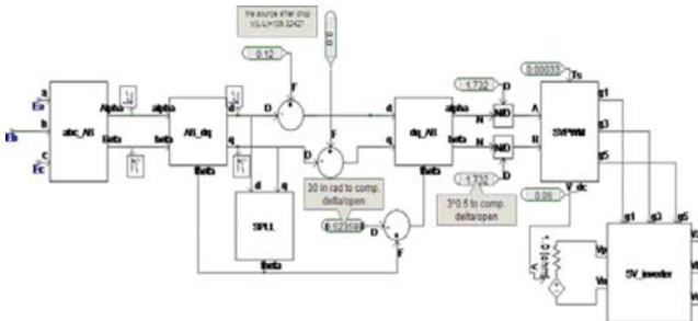
Fig. 5 Simulation of the control circuit of the DVR
