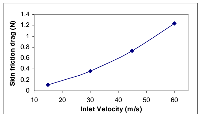
Fig. 8 Skin friction drag for different inlet velocity
