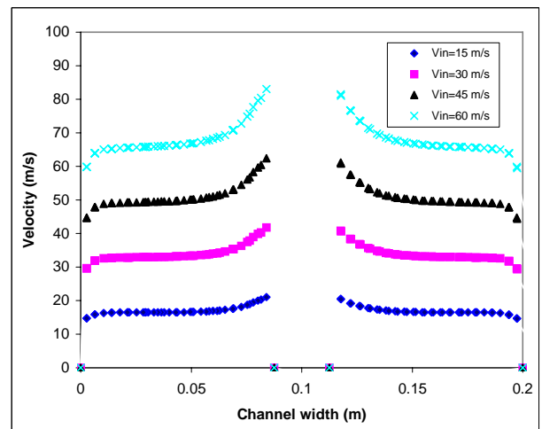
Fig. 4 Velocity magnitude profile at x = 0.25\text{m} behind the cylinder for high inlet velocities 15, 30, 45 and 60 m/s
