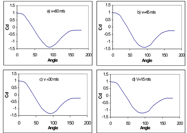
Fig. 6 Pressure distribution around a cylinder
