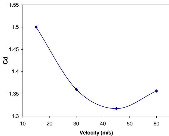
Fig. 5 Variation of drag coefficient ( C_d ) with Velocity
