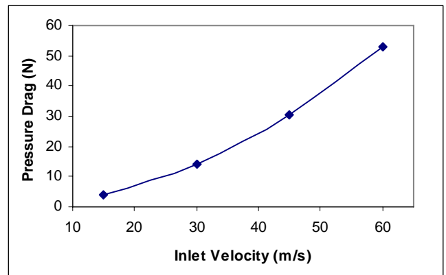
Fig. 7 Pressure drag for different inlet velocity
