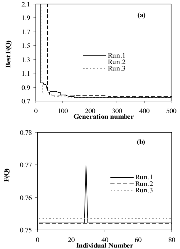
Fig. 5 (a) The best fitness value of chromosomes in three runs of DGA; (b) the fitness value of chromosomes at final generation
