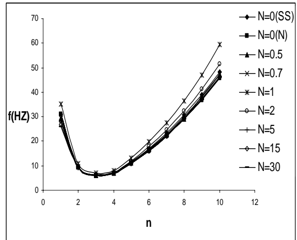
Fig. 3 Natural frequencies FG cylindrical shell associated with various power law exponent for C-C boundary condition.
