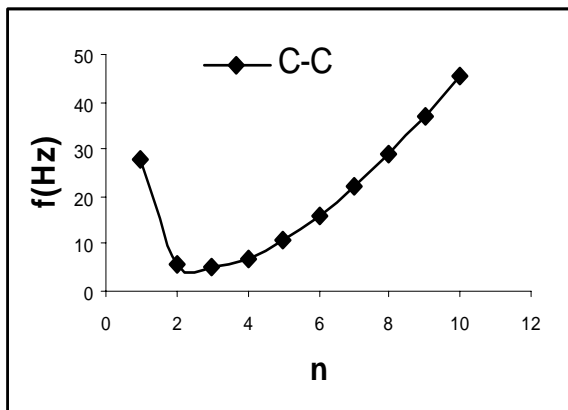
Fig. 2 Natural frequencies FG cylindrical shell associated with C-C boundary conditions. (m=1, h/R=0.002, L/R=20)
