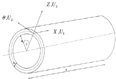
Fig. 1 Geometry of FGM cylindrical shell
