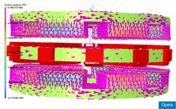
Fig. 7. Flux path in Slotless torus
