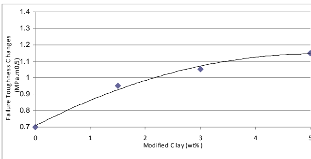
Fig. 6 failure toughness changes of nano composite per modified clay
