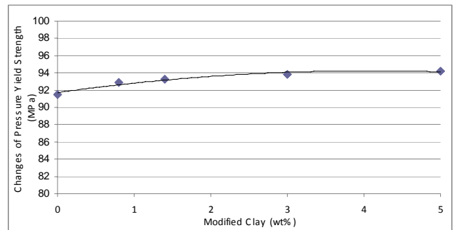
Fig. 3 Changes of pressure yield strength a nano composite per modified clay
