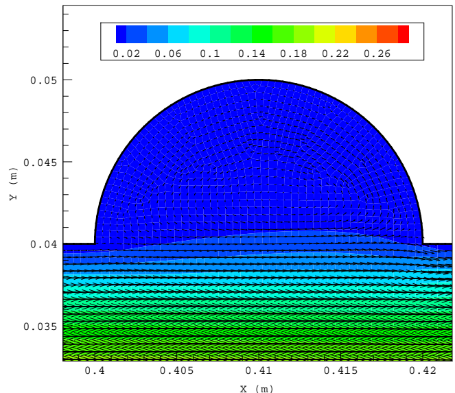
Fig. 3(b) Velocity vectors and velocity magnitude contours (m/s) inside a dimple with δ/D=0.5 on the 3-cavity channel
