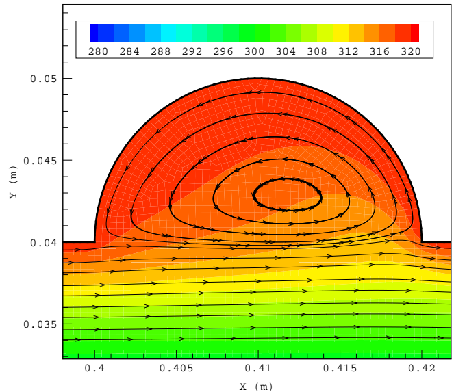
Fig. 3(a) Streamlines and temperature distribution (K) inside a dimple with δ/D=0.5 on the 3-cavity channel
