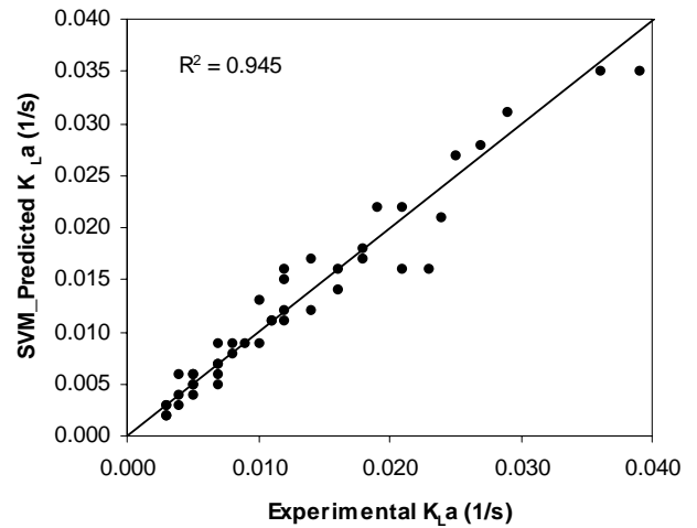
Fig. 2 Overall oxygen transfer coefficient by support vector machines versus experimental data.
