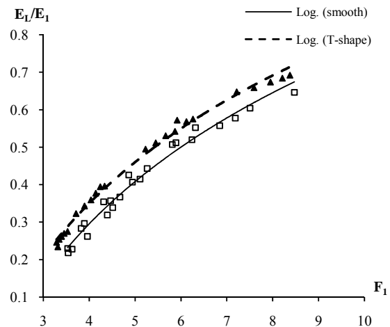
Fig. 11 Comparison between T-shape and smooth bed according to E_L/E_1
