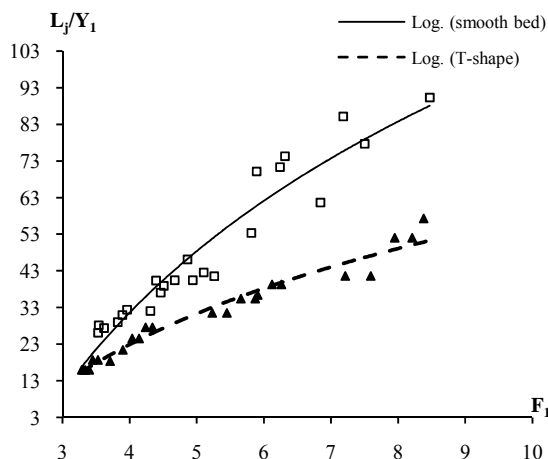
Fig. 10 Comparison between T-shape and smooth bed according to L_j/Y_1
