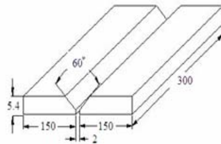
(a) Single 'V' butt joint (for GTAW)
