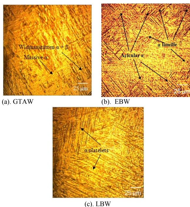
Fig.8 Optical micrograph of weld metals
