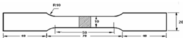
(c) Tensile specimen
