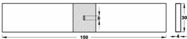
(b) Center cracked tension (CCT) fatigue specimen
