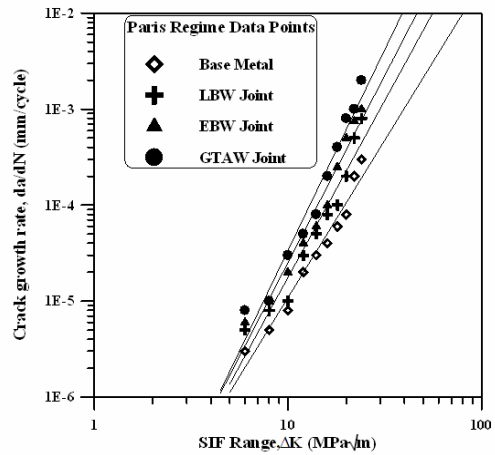
Fig.6 Effect of welding processes on fatigue crack growth rate
