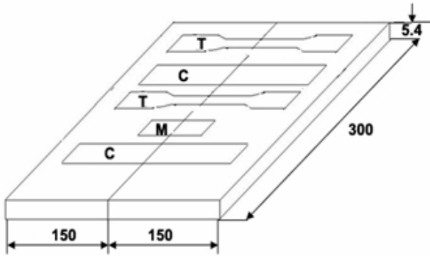
(a) Scheme of welding with respect to rolling direction and extraction of specimens (T-tensile, C-CCT and M- metallographic specimens)
