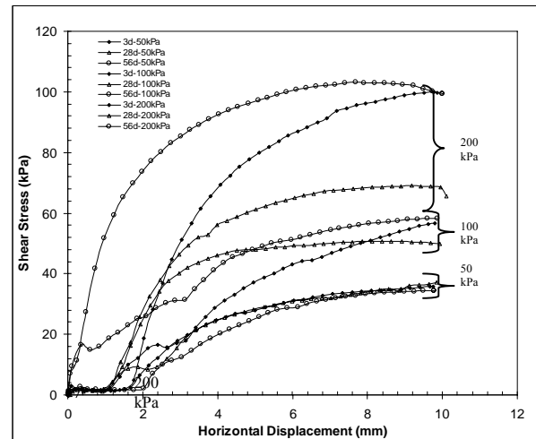
Fig. 6 Shear strength for columnar system specimens (10 % cement)
