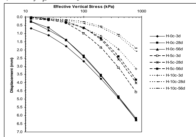
Fig. 1 Compression curve for all homogeneous specimens
