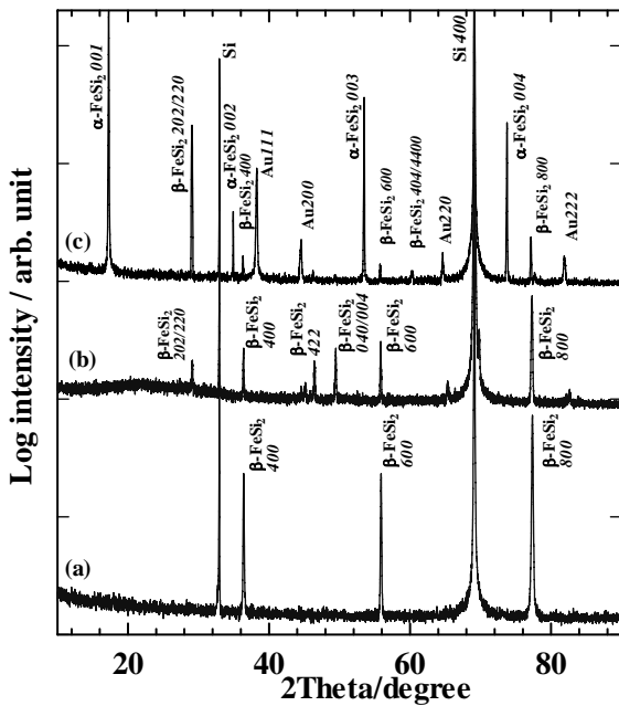
Fig. 1 XRD \theta - 2\theta scan profiles for the film on (a) Si(001) with \beta -FeSi 2 template, (b) 20nm-thick Cu coated Si(001), and (c) 40nm-thick Au-coated Si(001) wafers.
