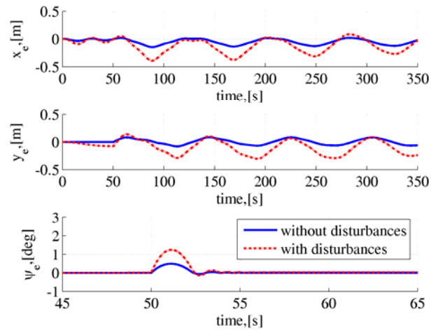
Fig. 5. Tracking errors (with and without disturbances) for circular tracking
