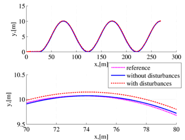
Fig.7. AUV reference and actual path (with and without disturbances) for sinusoidal tracking, (Plot in down: enlarged view)
