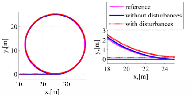
Fig. 4. AUV reference and actual path (with and without disturbances) for circular tracking, (right side plot: enlarged view)
