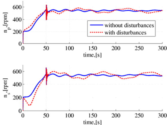
Fig. 9. Port side ( n_p ) and starboard side ( n_s ) thruster rotations (with and without disturbances) for sinusoidal tracking
