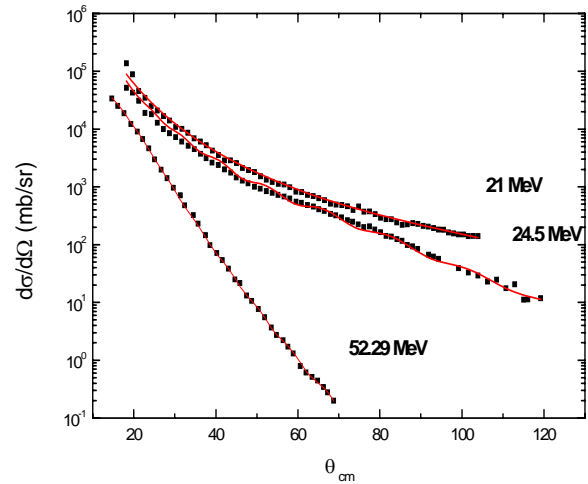
Fig. 3. The angular distribution of ^{14}\text{N} elastically scattered on ^{27}\text{Al} at energies 21, 24.5, 52.29 MeV respectively. The optical-model calculations are given by the solid curves while the experimental results are represented by dotted curves.
