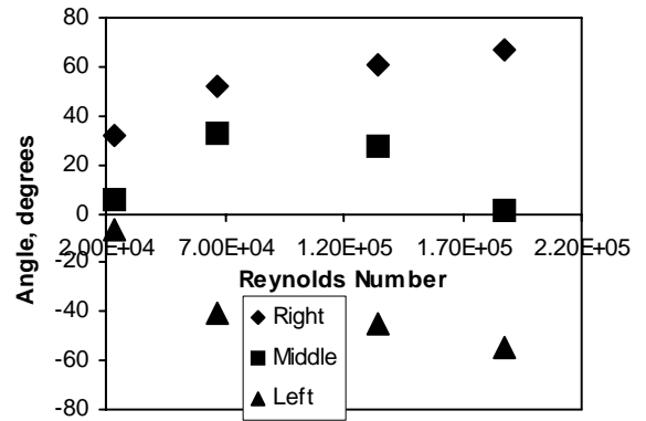
Fig. 11 Variation of Angle between Total Force and Wind Direction for Stacks in Side-by-side Configuration
