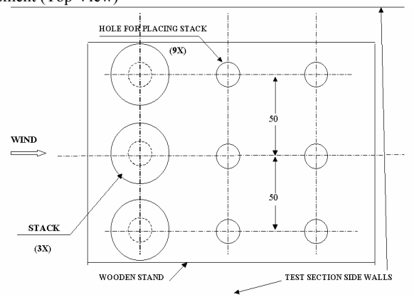
Fig. 2 Experimental Set Up for Stacks in Side-by-side Arrangement (Top View)
