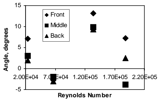
Fig. 7 Variation of Angle between Total Force and Wind Direction for Stacks in Along Wind Linear Configuration
