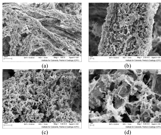
Fig.4 Scanning electronic micrographs of cigarette filter media after microbial colonisation: (a) cellulose acetate fibers (mag. \times 500), (b) a cellulose acetate fiber (mag. \times 2.50k), (c) microbial biofilm on a cellulose acetate fiber (mag. \times 1.00k) and (d) void spaces between microbial biofilms (mag. \times 5.00k).
