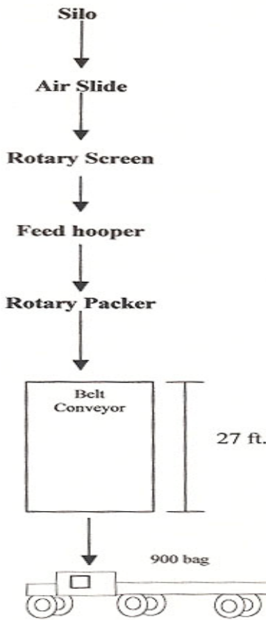
Fig.3 Flow diagram of proposed packing process of XYZ Ltd
