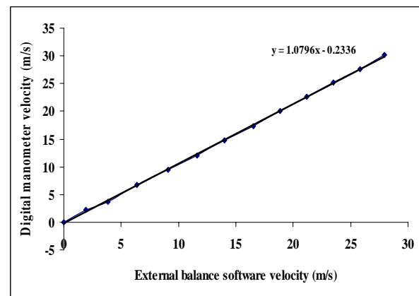
Fig.5. Flow velocity calibration for external balance
