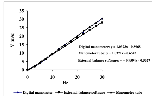
Fig.4. Free stream velocity vs. RPM controller speed.
