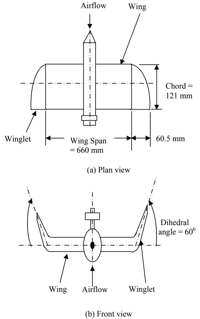
Fig.1. Schematic diagram of the aircraft model with winglet.
