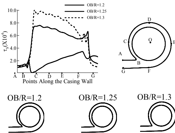
Fig. 15. Solid wall shear stress for different tongue geometries viz. OB/R = 1.2, OB/R = 1.25 and OB/R = 1.3.
