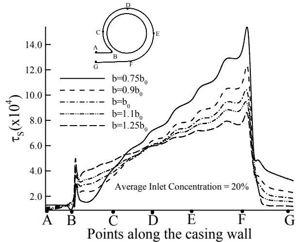
Fig. 16. Wall shear stress distribution along the casing wall for various casing widths viz. b = 0.75 b 0 , b = 0.9 b 0 , b = b 0 , b = 1.1 b 0 and b = 1.25 b 0 . These wall shear stresses for the solid phase are normalized w.r.t. \rho U_o^2 .
