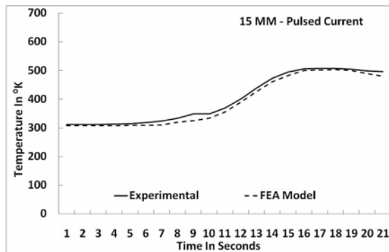
Fig. 7 (b) Experimental Vs FEA at 15 mm Pulsed Current
