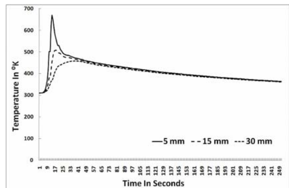
Fig. 6 (b) Pulsed Current Temperature profile
