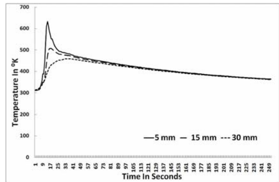
Fig. 6 (a) Constant Current Temperature profile
