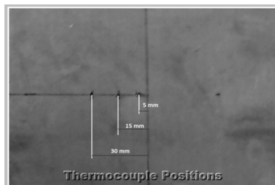
Fig. 2 Thermocouple positions
