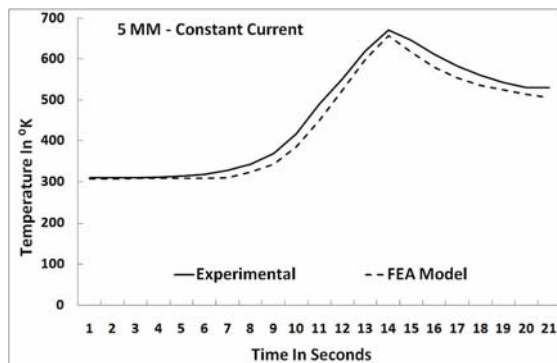
Fig. 8 (a) Experimental Vs FEA at 5 mm Constant Current
