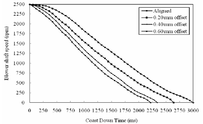
Fig. 2 CDT profile for parallel misalignment at 2500 rpm
