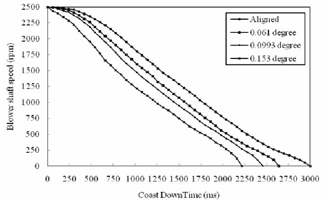
Fig. 3 CDT profile for angular misalignment at 2500 rpm
