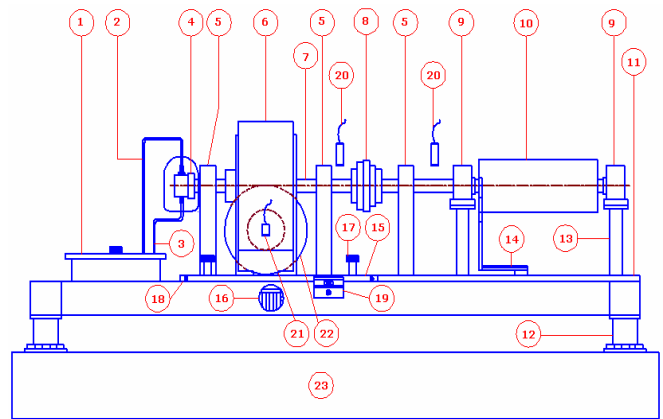
Fig. 1 Centrifugal Blower Experimental Test Rig
