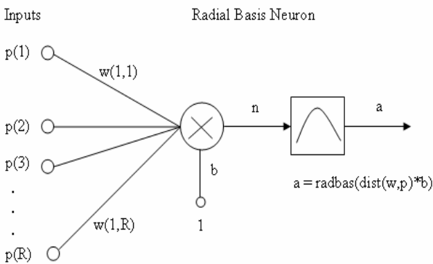
Fig. 5 Radial Basis Neuron Model
