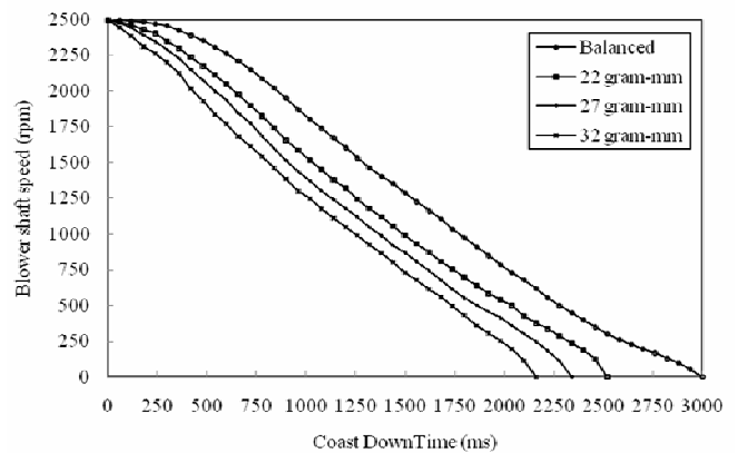
Fig. 4 CDT profile for unbalance at 2500 rpm
