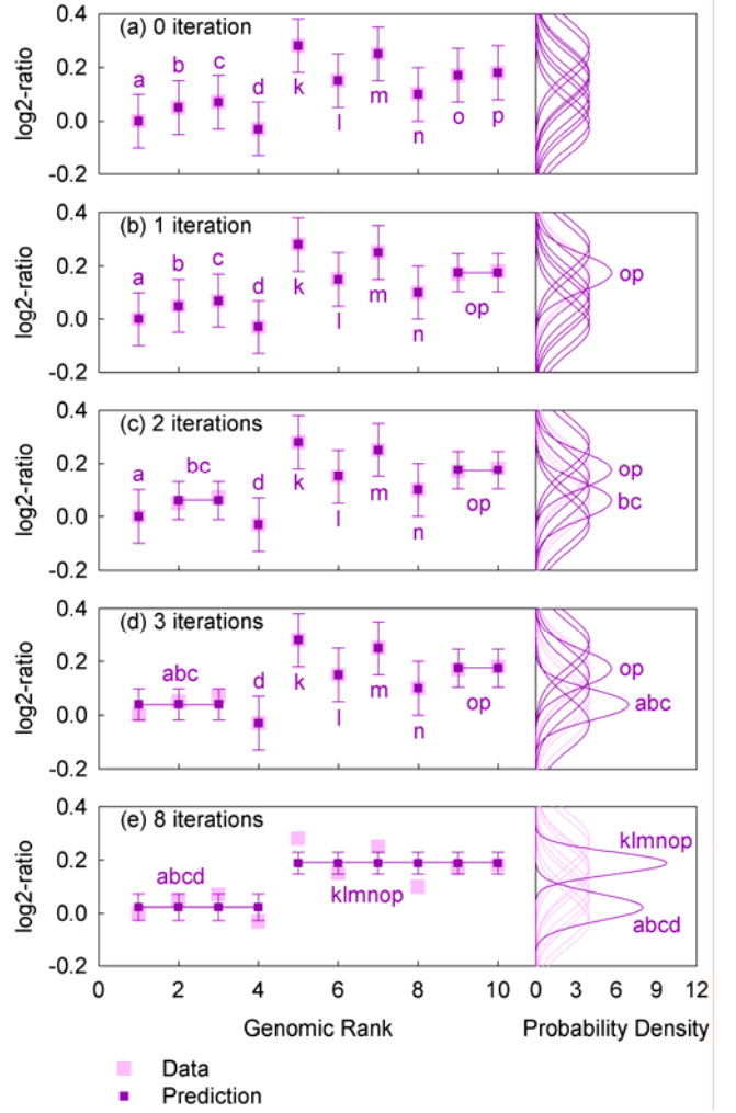
Fig. 1 Schematic illustration of PGM applied to genome segmentation. Frames on the left display the \log_2 -ratios of probes (data) and clusters (prediction at various stages) and those on the right display associated Gaussians. In (a), each piece of raw data is treated as a Gaussian with variance \tilde{\sigma} . In (b), data o and p, the nearest neighboring pair, are merged in the first iteration. (c) and (d) show second and third iterations, respectively. In (e), merging stops after eight iterations because the remaining cluster pair satisfies t \geq t_{min}
