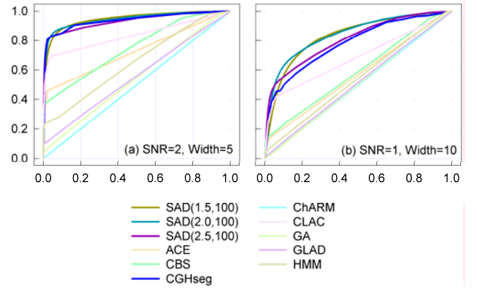
Fig. 2 ROC curves of \text{SAD}(1.5, 100) , \text{SAD}(2.0, 100) and \text{SAD}(2.5, 100) compared with the eight EPs in LJKP in two difficult situations, (\text{SNR}, \text{Width}) = (2, 5) in (a) and (1, 10) in (b)
