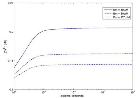
Fig. 4. Variation of calcium with time and Mobile buffer concentration Parameters: As stated in the Table I.
