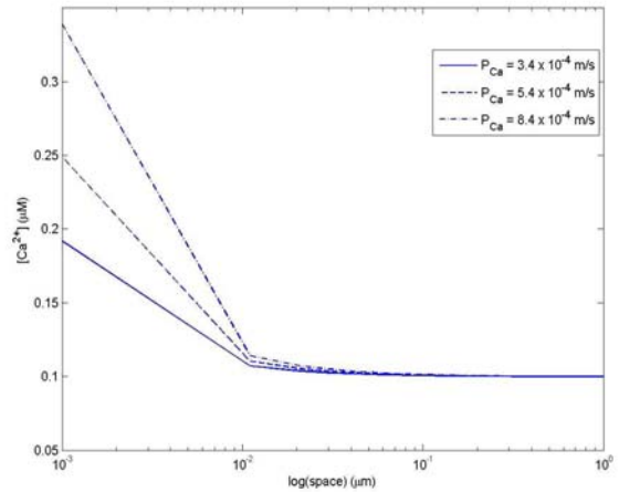
Fig. 3. Variation of calcium with space and calcium permeability. Parameters: As stated in the Table I.
