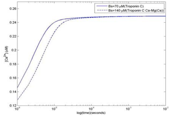
Fig. 7. Variation of calcium with time and Stationary buffer concentration Parameters: As in Table I.
