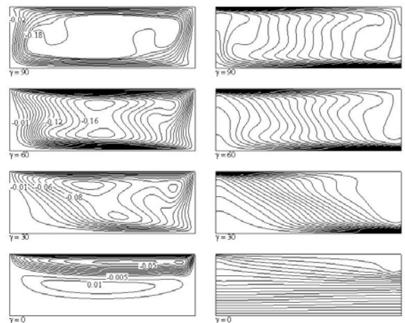
Fig. 4 Streamlines and isotherms for Ri = 10 , at \gamma = 0, 30, 60 and 90^\circ
