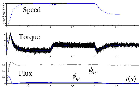
Fig.7 Results of the simulation of the completely discrete command: case where kd, and kq corresponds to places of roots being at the interior of the circle unit, without adaptation of rotor time constant.
