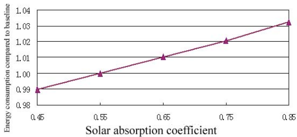
Fig. 3 Solar absorption coefficient vs total energy consumption
