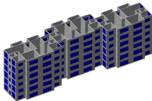
Fig. 1 The baseline building
