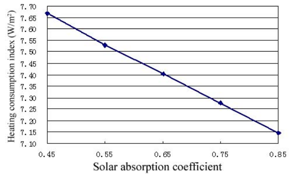
Fig. 4 Solar absorption coefficient vs heating consumption index
