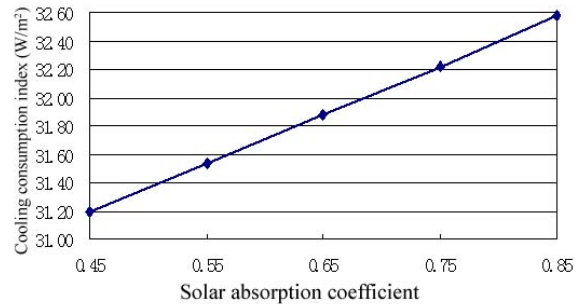
Fig. 5 Solar absorption coefficient vs cooling consumption index
