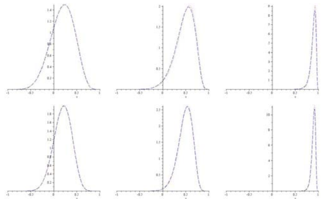
Fig. 2. Exact density of R from Equation (2): dotted line, and mixture of the approximate density functions specified by (13) and (15): dashed line for \rho = 0.2, 0.5 and 0.9 (left to right) and sample sizes 15 and 25 (top and bottom graphs).
