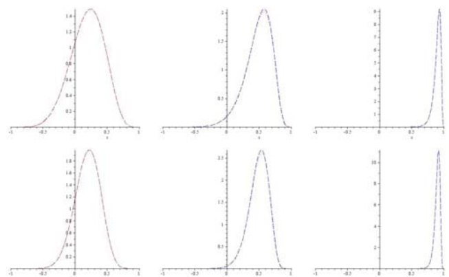
Fig. 3. Exact density of R from Equation (2): dotted line, and the approximate density from Equation (16) with d = 7 : dashed line) for \rho = 0.2, 0.5 and 0.9 (left to right) and sample sizes 15 and 25 (top and bottom graphs).
