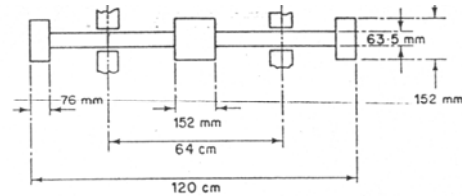
Fig. 2 Rotor with all disks
