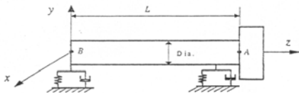
Fig. 6 Rotor with end disk position
