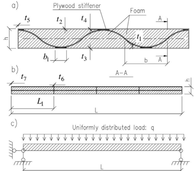
Fig. 1 The panel with curved plywood ribs: a – cross section, b – longitudinal section, c – structural analysis scheme
