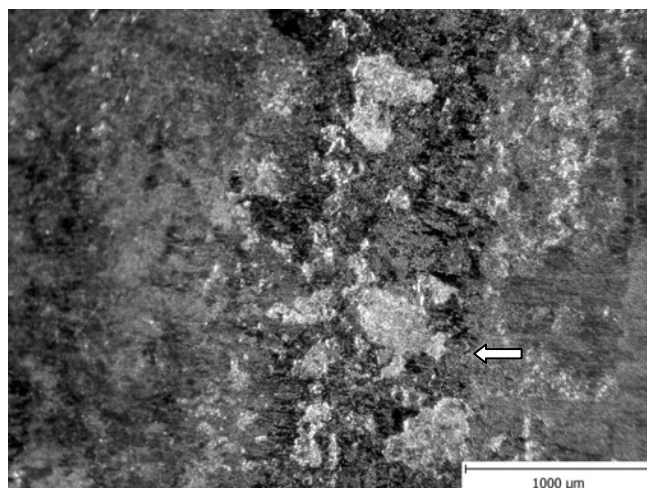
Fig. 14 Areas with seizing. Nitrided EA4T specimen
