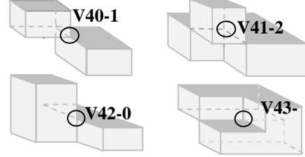
Fig. 4 Four possible vertex configurations for V4
