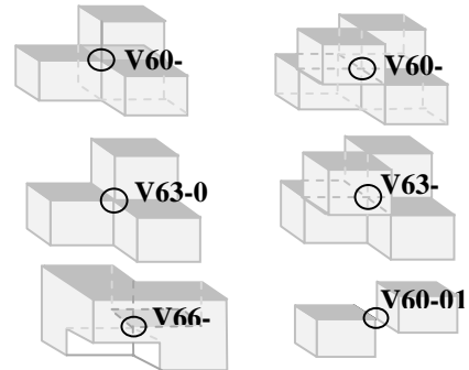
Fig. 6 Configurations a vertex having 6 edges in OPP
