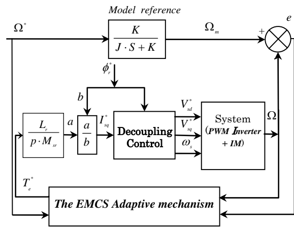
Fig. 5 Configuration of the control system
