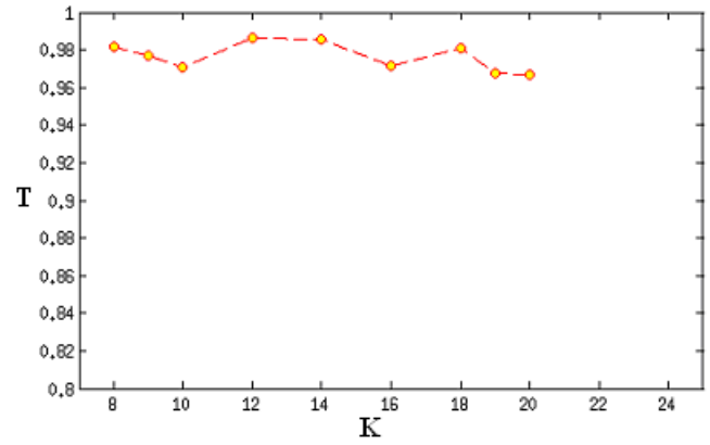
Fig. 2: Trustworthiness of LPC on Swiss-roll data set
