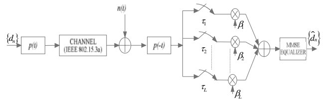
Fig. 3 UWB SRAKE-MMSE receiver structure
