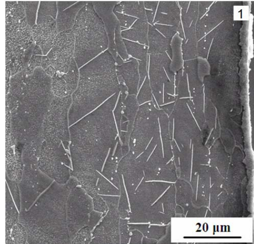
Fig. 2 Coarse needles of Fe 4 N nitrides
