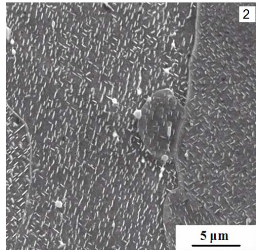
Fig. 3 Fine Fe 16 N 2 nitrides regularly dispersed in ferritic matrix
