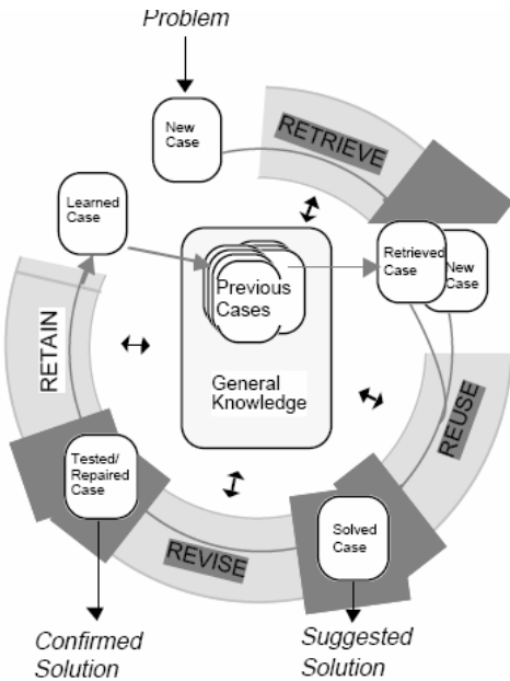
Fig.1 CBR Cycle
